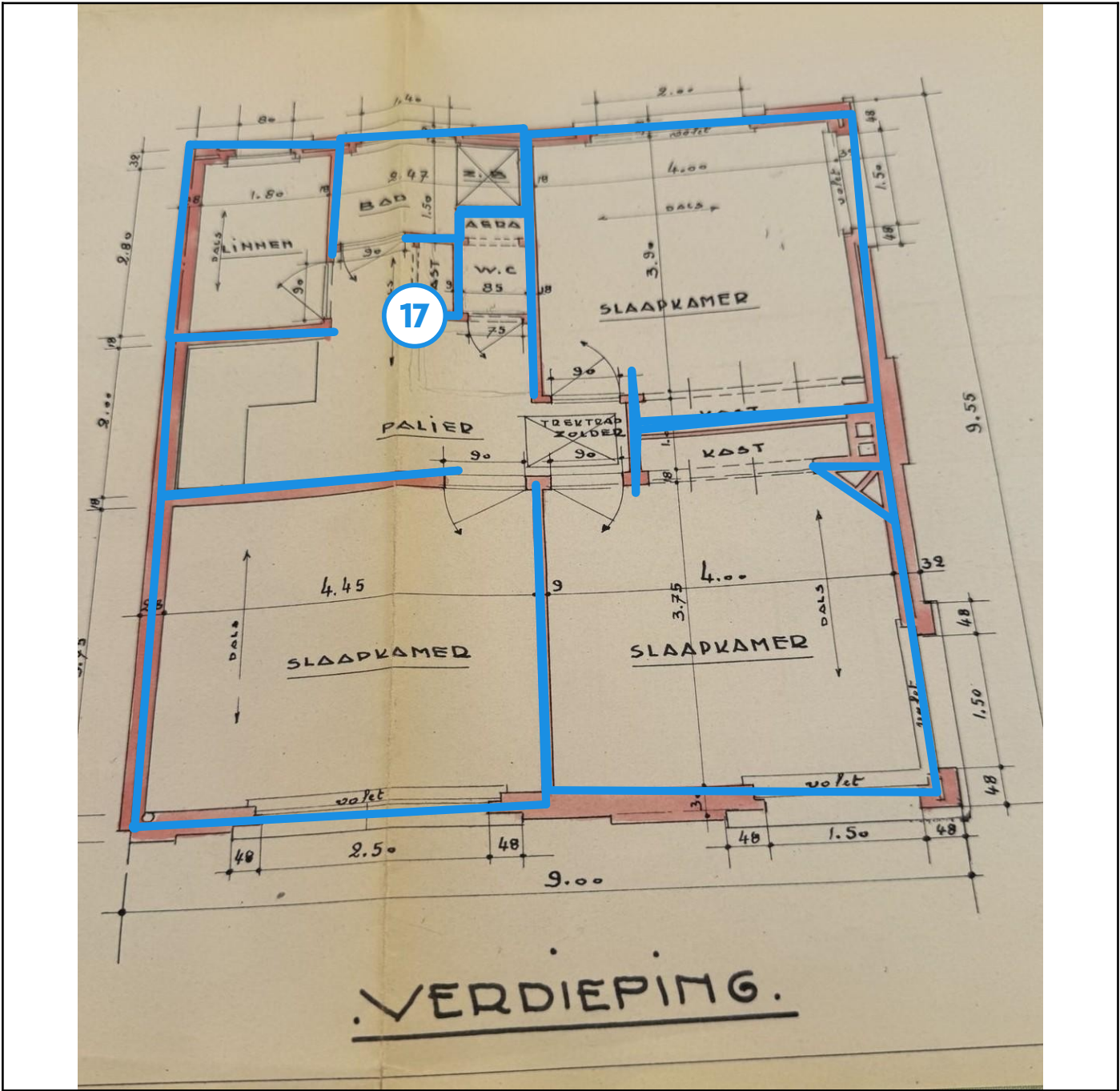
Legende van plan 1.6: Plan verdieping
