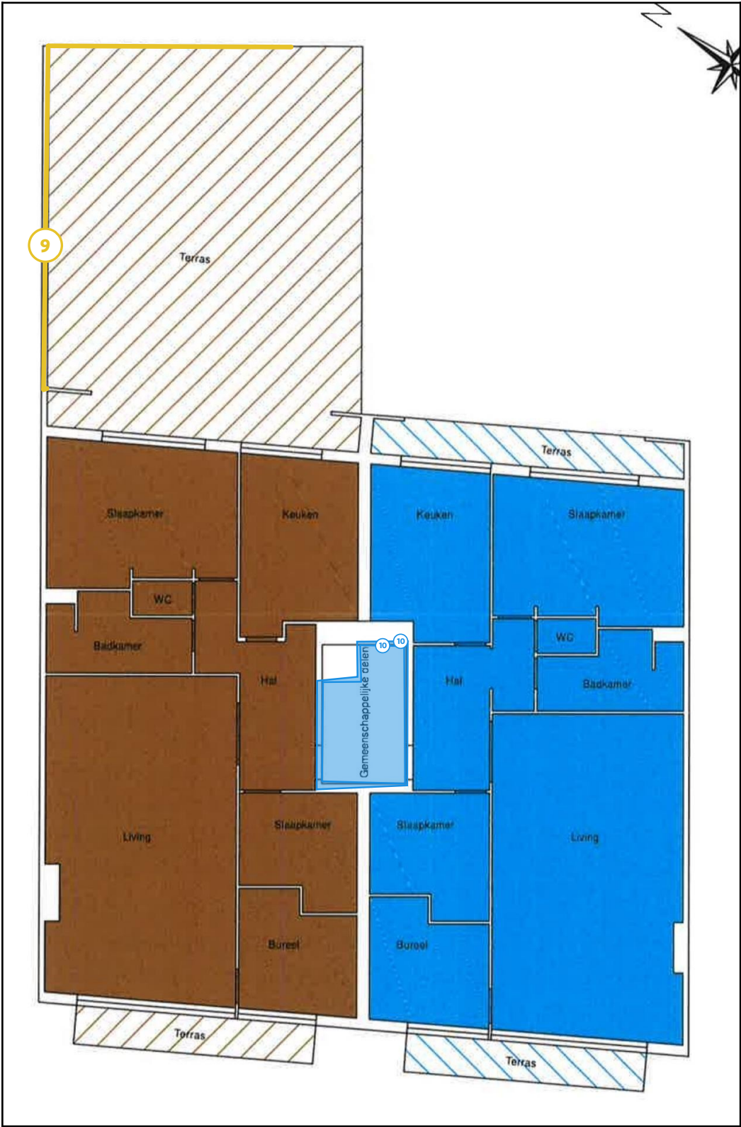
Legende van plan 1.3: Verdieping +1
